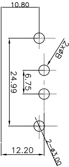
PCB LAYOUT
