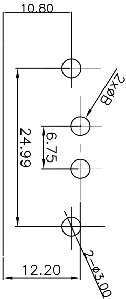
PCB LAYOUT
